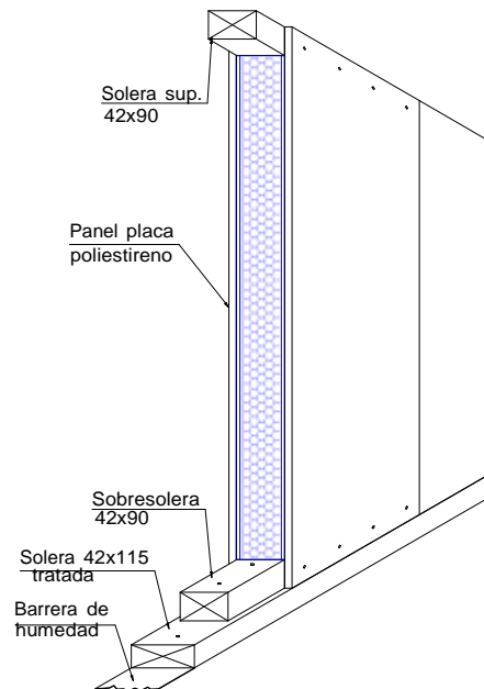
Fig. 1 Detalle panel
